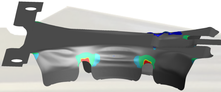
Forecasting of cracks and folds with Stampack
